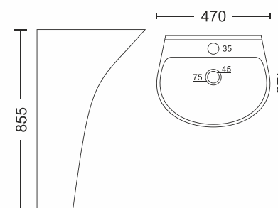
BOLSA 3003 470 x 425 x 855mm
