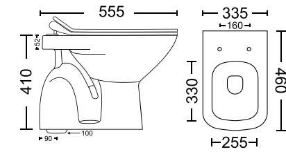
RECT 8105 555 x 335 x 410mm
