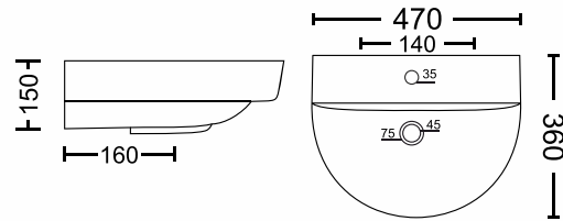
OSCAR 4022 470X360X150mm 18X14 Inch (Approx)
