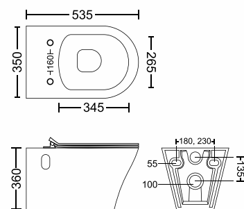
POLAR 2015 535 x 350 x 360mm
