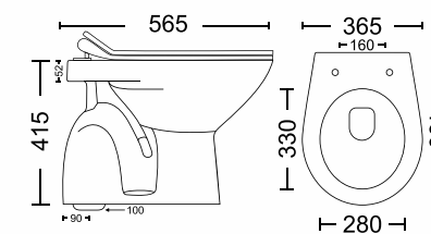
KEL 8106 565 x 365 x 415mm
