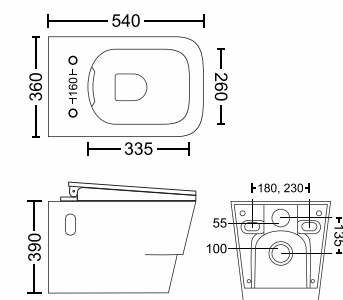
ALICE 2017 540 x 360 x 390mm
