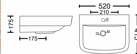
WILLIAM 4023 520X415X175mm 20X16 Inch (Approx)
