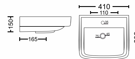
VIGGO 4025 410X365X150mm 16X14 Inch (Approx)
