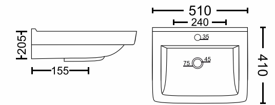
OLIVER 4024 510X410X205mm 20X16 Inch (Approx)
