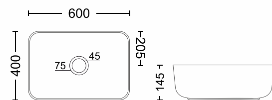
DOVER 7029 600 x 400 x 145mm 24 x 16 Inch (Approx)
