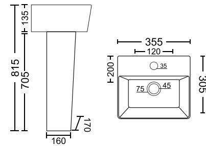
MARIT-BRUNO BWB 7008 + BPD 6004 355x305x815mm 14 x 12 Inch (Approx)
